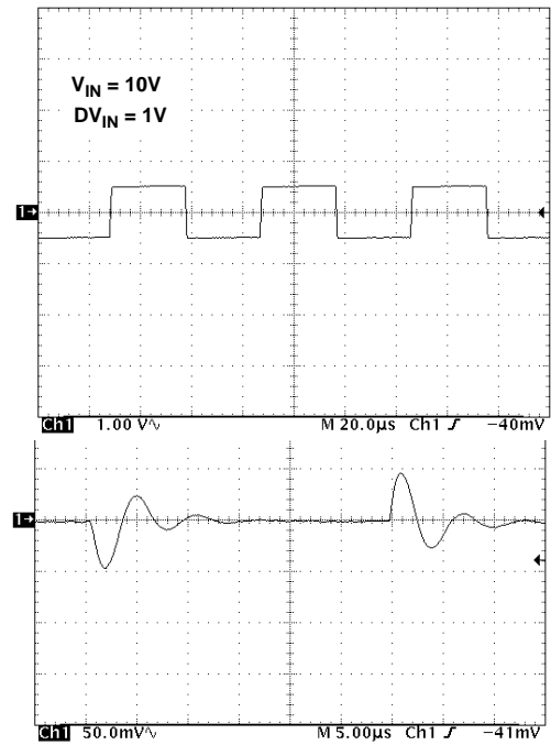
FIGURE 52. LINE TRANSIENT RESPONSE, 0.001µF LOAD CAPACITANCE
