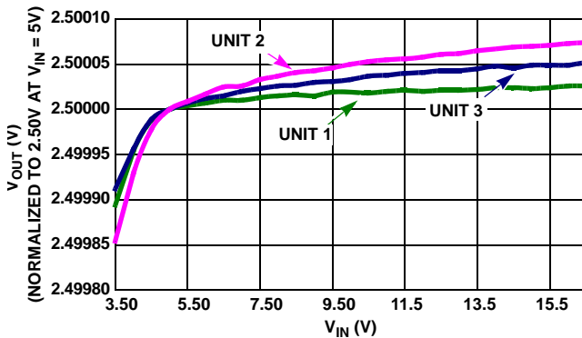
FIGURE 18. LINE REGULATION
